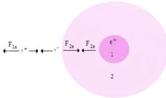
Fig4: Acceleration the electron and positron according to Newton's second law
