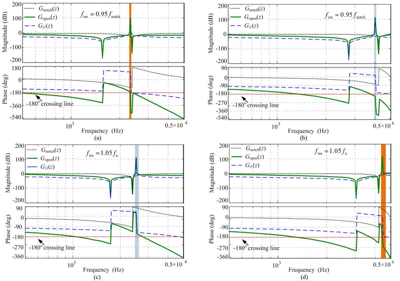
Fig. 8. Bode plots of the open-loop system with different resonant frequencies in case of ICF control: (a) ICF II: C_f = 4.7 \mu\text{F} with a +10% variation of capacitance, f_n > f_{res} , f_n = 2385 \text{ Hz} ; (b) ICF III: C_f = 1.5 \mu\text{F} with +10% variation of capacitance, f_n > f_{res} and f_n = 4222 \text{ Hz} ; (c) ICF II: C_f = 4.7 \mu\text{F} with -10% variation of, f_n < f_{res} and f_n = 2385 \text{ Hz} ; (d) ICF III: C_f = 1.5 \mu\text{F} with -10% variation of capacitance, f_n < f_{res} and f_n = 4222 \text{ Hz} .
