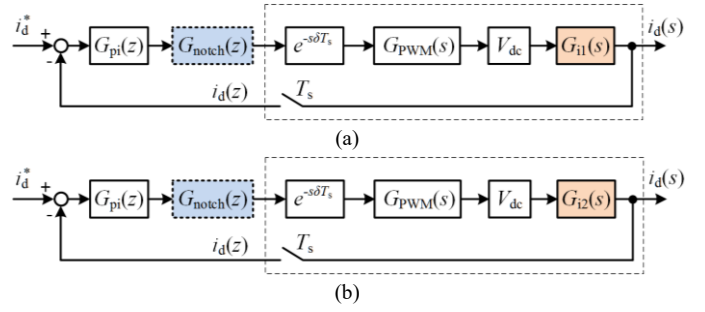
Fig. 2. Closed-loop current control system using a digital notch filter based active damping for the PWM converter with an LCL filter, where i_d is the d -axis component of the feedback current in the dq reference frame: (a) using inverter-side current feedback control (ICF) and (b) using grid-side current feedback control (GCF).
