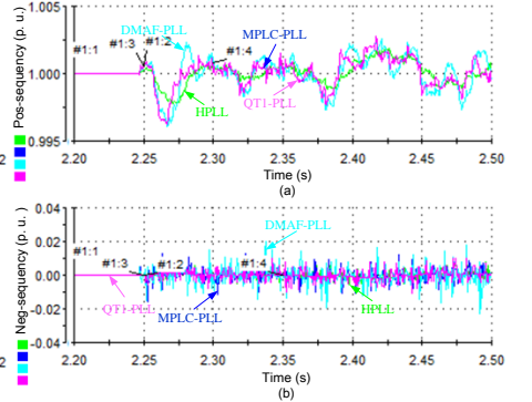
Fig. 31. Estimated pos. and neg. sequence amplitudes under noise contaminations.
