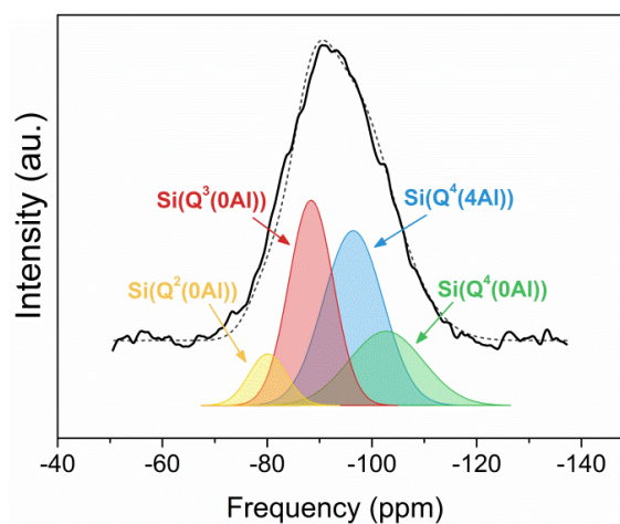
Figure 2 Example of Si(Q n (kAl)) unit distribution in glass, simulated (dashed, black line) from 29 Si MAS NMR spectrum of glass sample (solid, black line).
