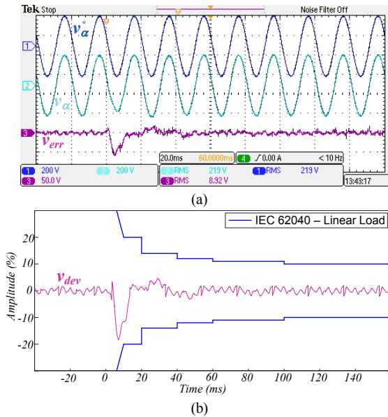
Fig. 18. Linear step load changing (0 – 100%): (a) reference (200 V/div), real (200 V/div), and capacitor voltage error (50 V/div) ( \alpha -axis); (b) Dynamic characteristics according to IEC 62040 standard for linear loads.
