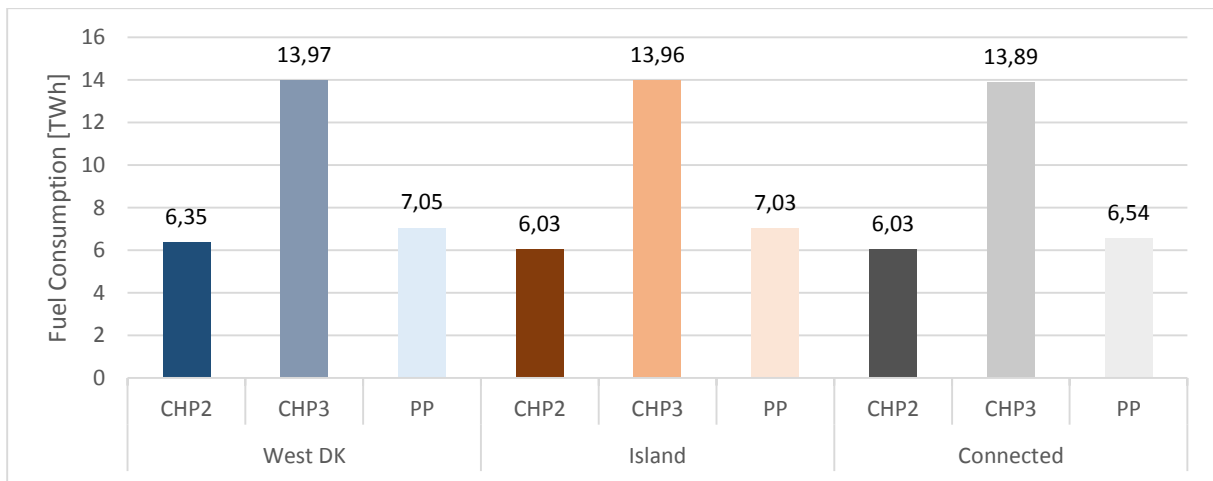
Figure 6. Fuel consumption for decentral CHP plant (CHP2), central CHP plant (CHP3) and power plants (PP), in the three models in analysis 2: single entity (West DK), regions as islands (Island), and interconnected regions (Connected)
