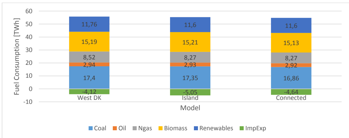
Figure 7. Net Total Fuel Use in the three models in analysis 2: single entity (West DK), regions as islands (Island), and interconnected regions (Connected)
