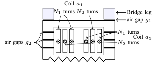
Fig. 10. Integrated inductor with split winding arrangement.
