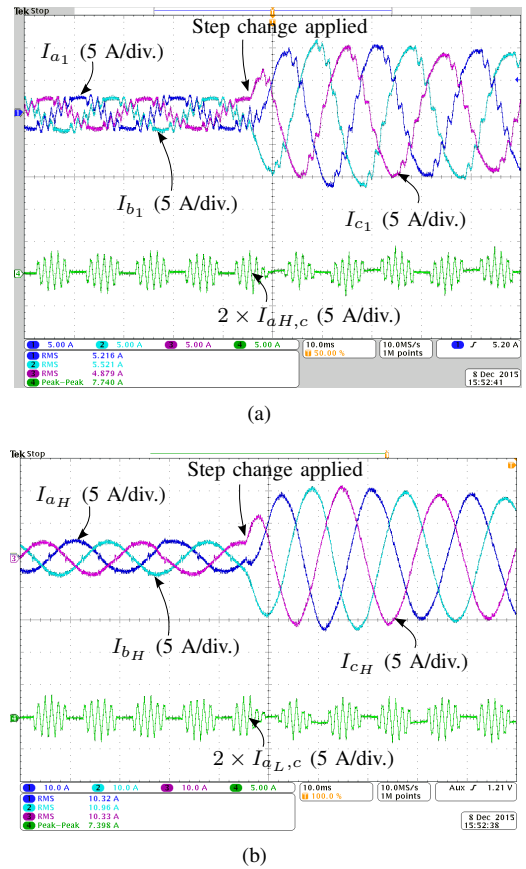
Fig. 16. Experimental waveforms for a step response when the reference current was changed from 0.25 pu to 1 pu. (a) Ch1: I_{a1} , Ch2: I_{b1} , Ch3: I_{c1} , and Ch4: I_{aH,c} . (b) Ch1: I_{aH} , Ch2: I_{bH} , Ch3: I_{cH} , and Ch4: I_{aL,c} .
