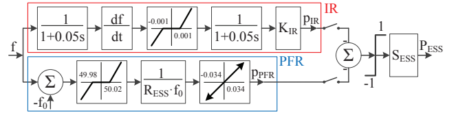
Fig. 7. Block diagram of the ESS control for IR and PFR services.
