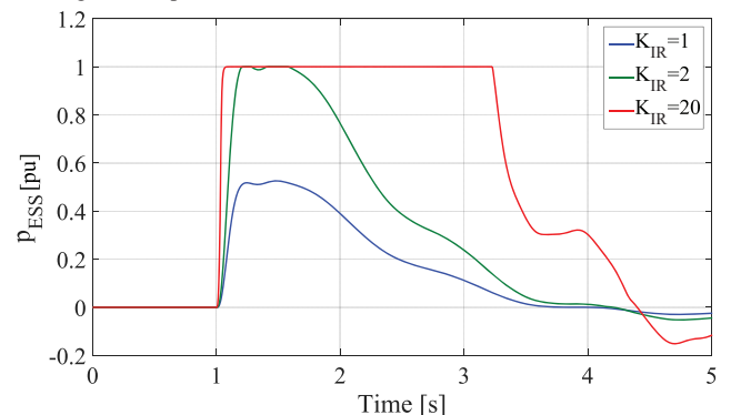
Fig. 10. The ESS power output ( p_{ESS} ) for selected K_{IR} and for power change of 175 MW.
