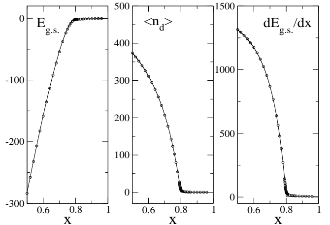
FIG. 2. Transition from O(6) to U(5) . The ground state energy (left panel), expectation value of the n_d (central panel), and derivative of the ground state energy (right panel) are presented as a function of the control parameter x for a system with 1000 bosons. The exact results are represented by circles and the mean field results by a full line.
