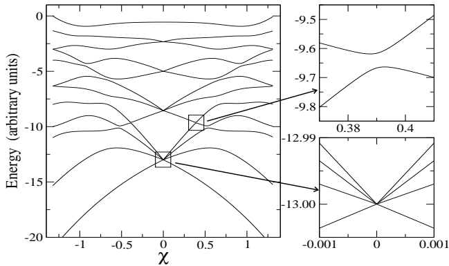
FIG. 4. Transition from \overline{SU(3)} to SU(3) through the O(6) limit. All 0^+ eigenstates of the Hamiltonian (8) for a system with N = 9 bosons are represented as a function of the control parameter \chi . The right panels show in a larger scale the level repulsion of two close levels at \chi \neq 0 (right-top panel) and the level crossing at \chi = 0 (right-bottom panel).
