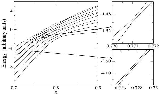
FIG. 3. Ten lowest 0^+ states in the transition from U(5) to SU(3) for N = 50 bosons as a function of x . On the right panels we show in an enlarged scale two examples of level repulsion.
