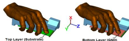
Fig. 14. Different placements of the proposed antenna in data mode.
