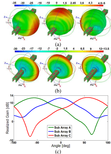
Fig. 5. Radiation patterns of proposed antenna package at 21.5 GHz for, (a) single elements, (b) sub arrays at 0^\circ scanning angle, and (c) converge space of the sub arrays with realized gain values.
