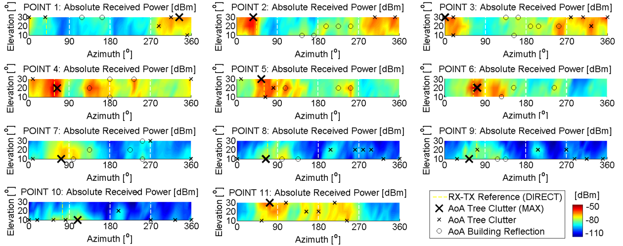
Fig. 4. Measurement results for all the considered positions: AoA and directional absolute received power values.
