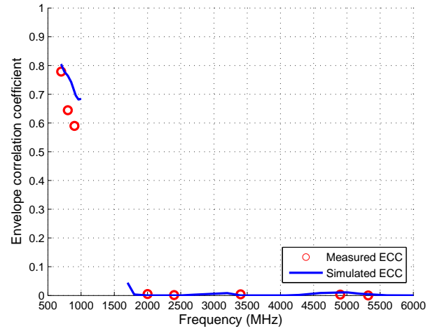
Fig. 6: Measured and simulated envelope correlation coefficient.
