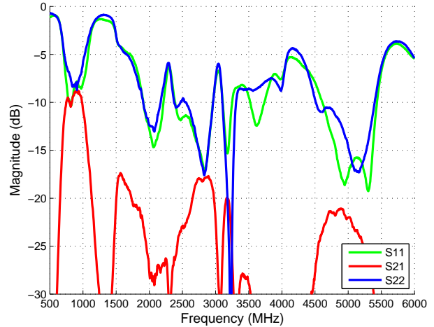
Fig. 3: Measured S-parameters of the proposed antennas.
