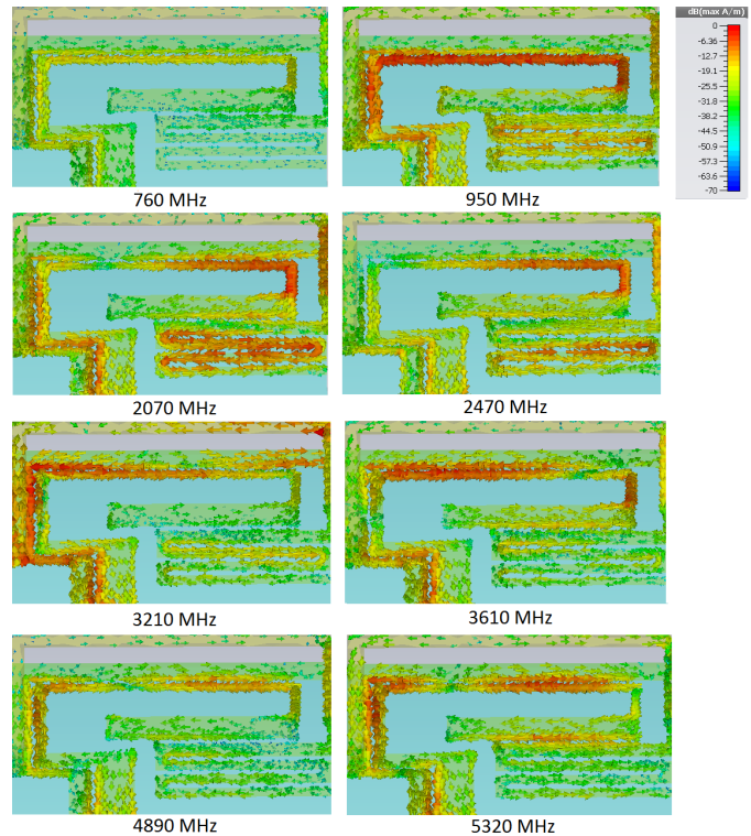
Fig. 4: Current distribution for one of the antennas.
