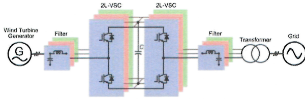
Fig. 8. 2L-VSC BTB voltage source converter for WTSs.
