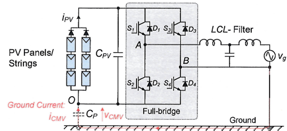
Fig. 10. Single-phase full-bridge PV inverter.
