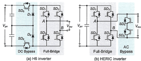
Fig. 11. Two transformerless PV inverters (H6 and HERIC) [41], [42]: (a) H6 inverter and (b) HERIC inverter.
