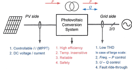
Fig. 3. Demands to PV power conversion systems.
