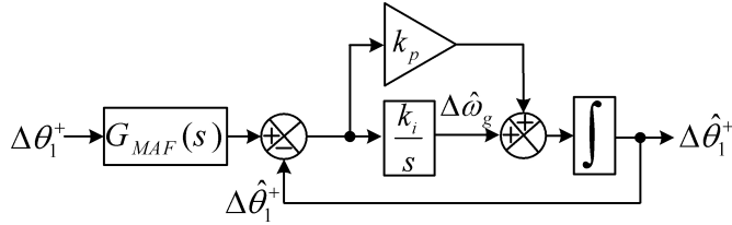
Fig. 4. Small-signal model of the PMAF-PLL in the s -domain.
