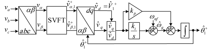
Fig. 9. Schematic of the SVFT-PLL.
