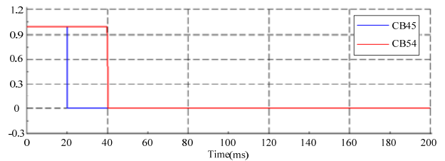
Fig. 11. States of CBs with normal distance protection.
