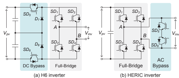
Fig. 8. Two transformerless PV inverters (H6 and HERIC) [41], [42]: (a) H6 inverter and (b) HERIC inverter.
