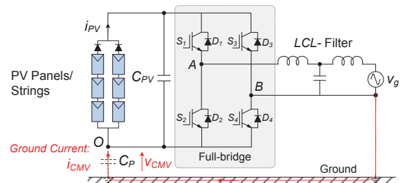
Fig. 7. Single-phase full-bridge PV inverter.
