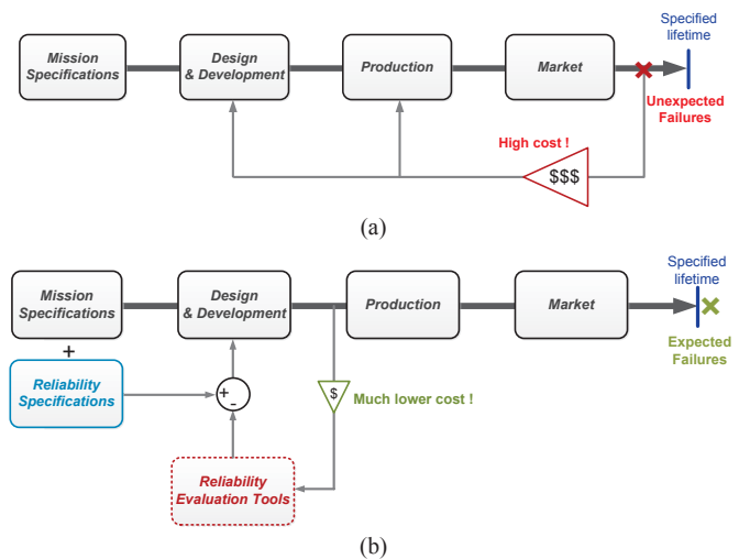
Fig. 1. Reliability improvement approaches for power electronics products: (a) typical flow in the past and (b) new flow in the future.
