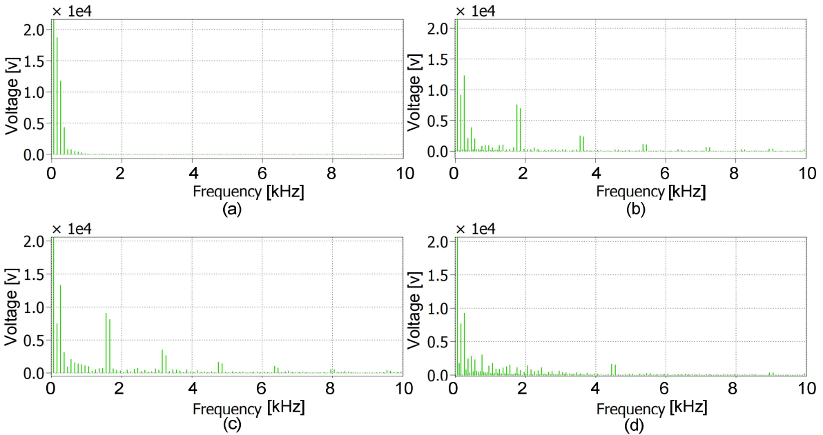
Fig. 8 Harmonic Spectrum of the output voltages where: (a) PSC-PWM, (b) NLC, (c) NLC+PWM, and (d) NLC+CRG modulation methods were used.
