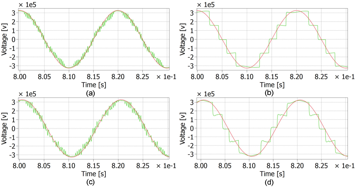
Fig. 5 Output voltage waveform of a phase of the MMC when: (a) PSC-PWM, (b) NLC, (c) NLC+PWM and (d) NLC+CRM modulation technique has been used.
