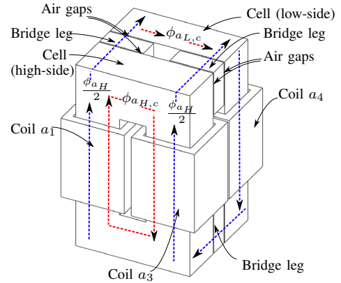
Fig. 5. Magnetic structure of the proposed integrated inductor.
