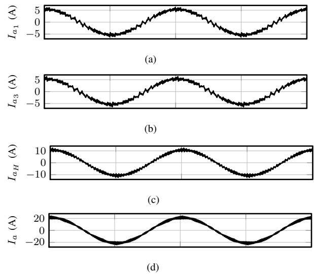
Fig. 14. Simulated current waveforms of phase a at rated operating conditions. (a) Output current VSC 1 ( I_{a_1} ), (b) Output current VSC 3 ( I_{a_3} ), (c) Resultant current of the high side converter group ( I_{a_H} ), (d) Line current I_a .
