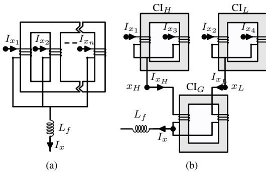
Fig. 2. Various arrangements of the filters for the parallel interleaved VSCs. (a) CI with N -limb core structure, (b) Whiffletree configuration using the two limb CIs. The subscript x represents phases x = \{a, b, c\} .
