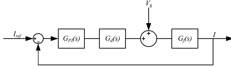
Fig. 3 Grid current controller including the grid voltage feed forward and delay introduced by the converter
