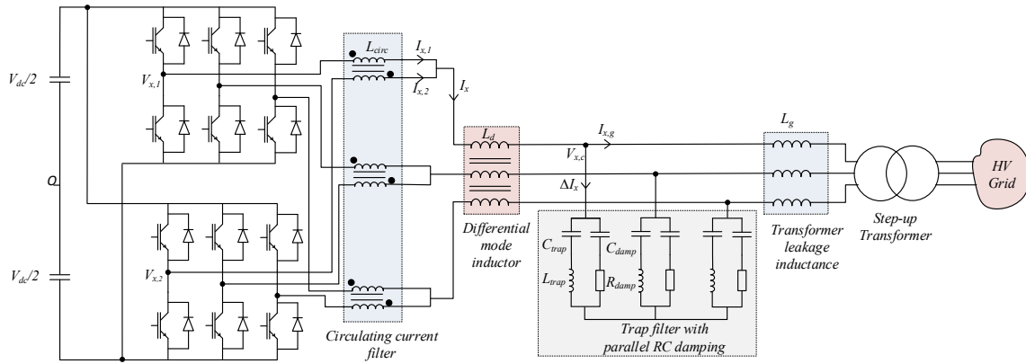
Fig. 1 Two parallel converters with trap filter connected to grid
