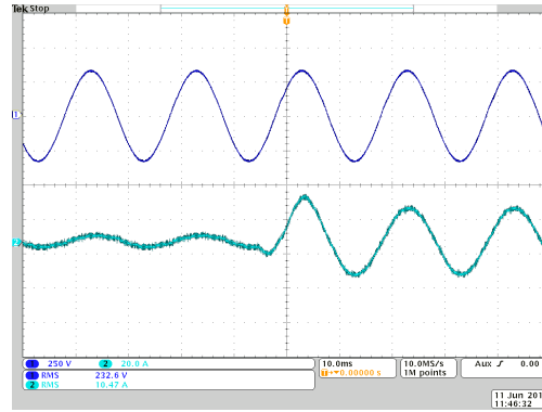
Fig. 18 Converter current feedback: Experimental results for a step change from 20% to 100% load; Ch1 (blue) - phase A grid voltage; Ch2 (light blue) - phase A grid current ( I_{g,A} );
