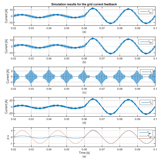
Fig. 9 Simulation results - Grid current feedback: for a step change from 20% to 100% load; (a) - phase A current VSC1; (b) - phase A current VSC2; (c) - Circulating current ( I_c ) between Phase A VSC1 and Phase A VSC2; (d) - Total Current ( I_{x,A} ); (e) - normalized grid current ( I_{gA} ) and voltage ( V_{gA} )
