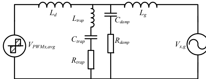
Fig. 2 Trap filter with parallel RC damping
