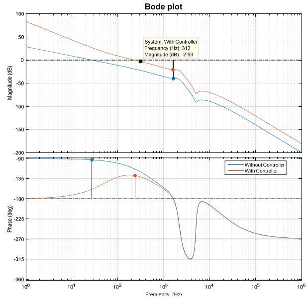
Fig. 5 Bode plot of the system of the transfer function where the output is the grid current; without (blue line) and with (red line) controller
