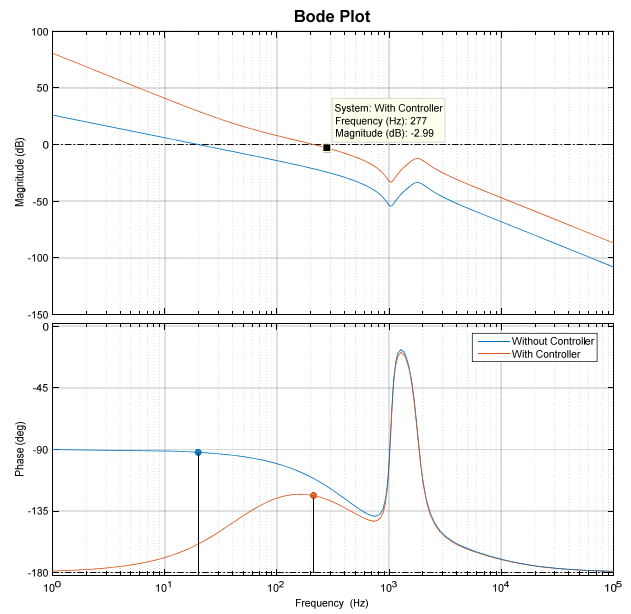
Fig. 7 Bode plot of the system without (blue line) and with (red line) controller
