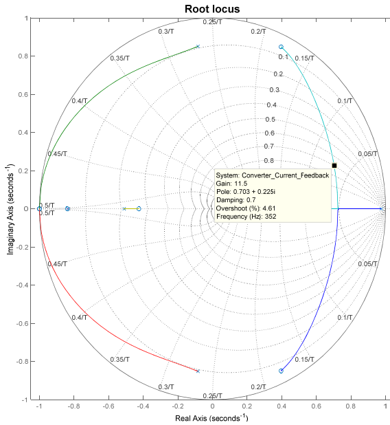
Fig. 6 Root locus plot of the transfer function in (8)
