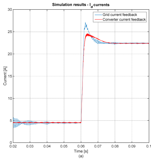
Fig. 10 Simulation results: I_d (a) and I_q (b) components of the grid current for a step change in the load from 20%
