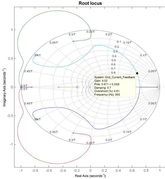
Fig. 4 Root locus plot of the transfer function where the output is the grid current
