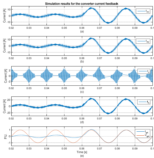
Fig. 8 Simulation results - Converter current feedback: for a step change from 20% to 100% load; (a) - phase A current VSC1; (b) - phase A current VSC2; (c) - Circulating current ( I_c ) between Phase A VSC1 and phase A VSC2; (d) - Total Current ( I_{x,A} ); (e) - normalized grid current ( I_{gA} ) and voltage ( V_{gA} )
