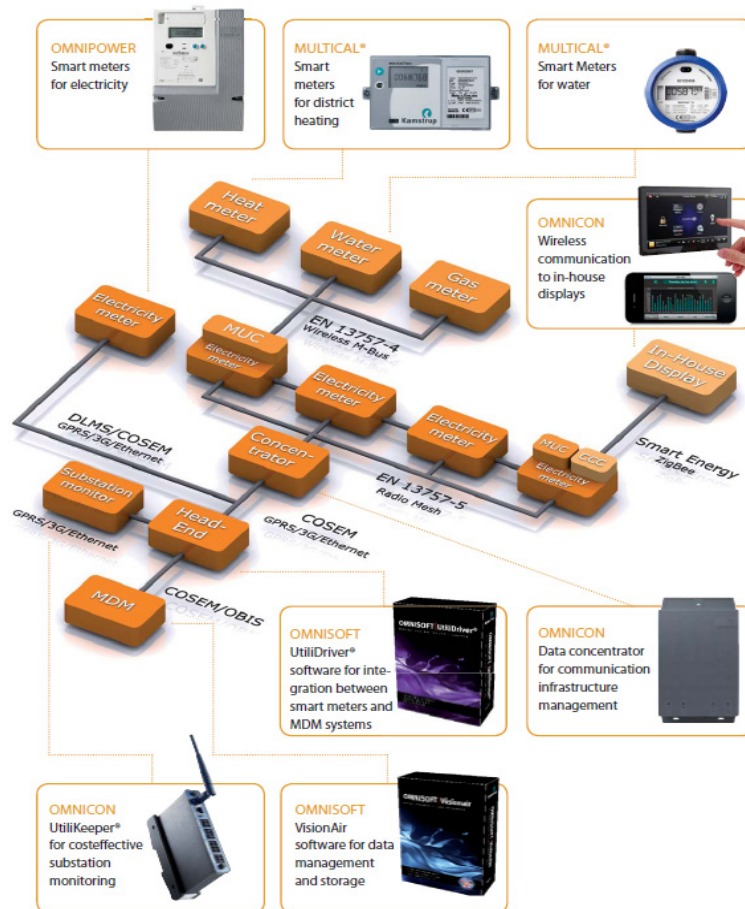
Fig. 4. Configuration of Kamstrup OMNIA system
