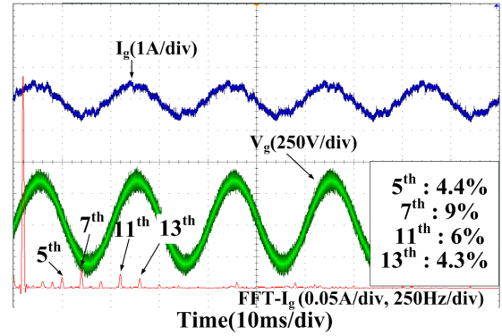
Grid Voltage ( V_g ) & Grid Current ( I_g )
