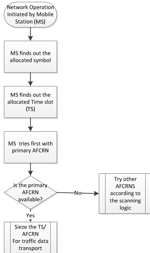
Figure 5: Sequence of the processes to hunt for AFCRN and seize the time slot for data transport
