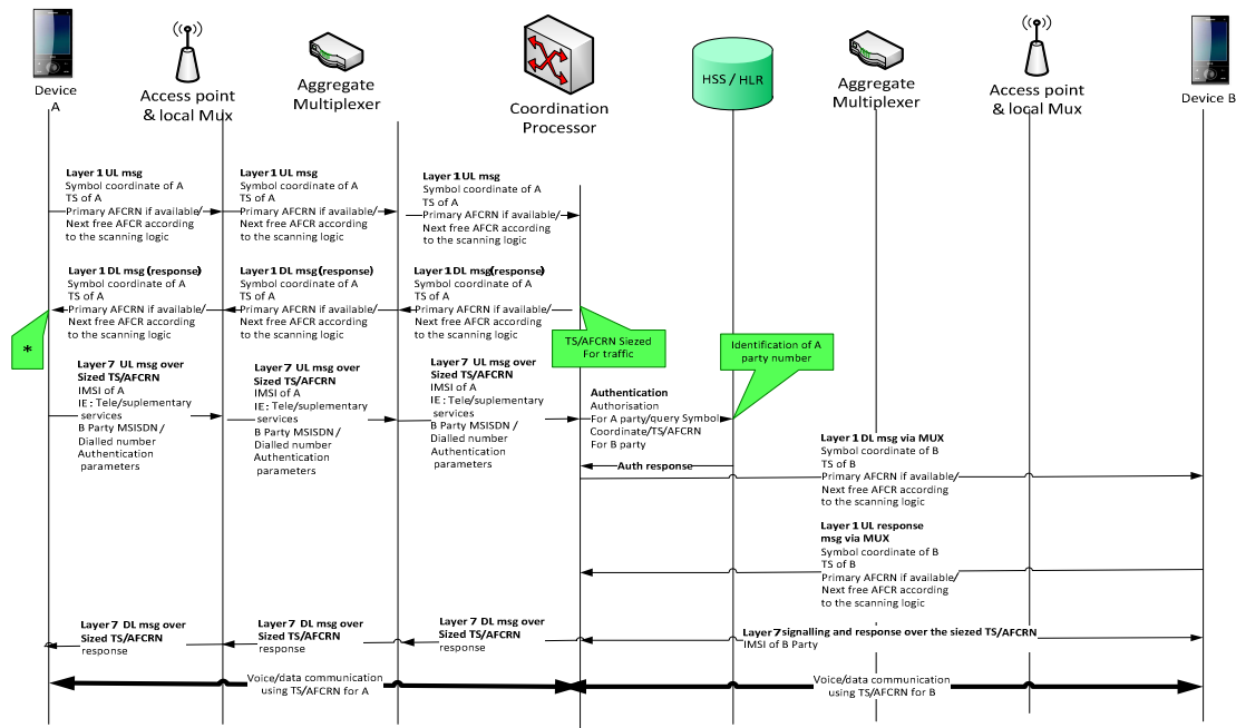
Figure 26: End2End call flow between 2 mobile devices actuated by the Coordination Processor
