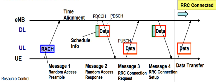
Figure 36: Synchronisation and the Random Access process for the LTE Access layer
