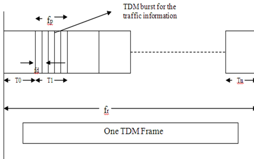
Figure 3: TDMA frame
