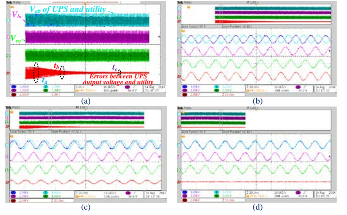
Fig. 21. Synchronization process between v_{ab\_utility} and v_{ab\_UPS} under linear load condition. (a) Overall process. (b) Details at t_a . (c) Details at t_b . (d) Details at t_c .
