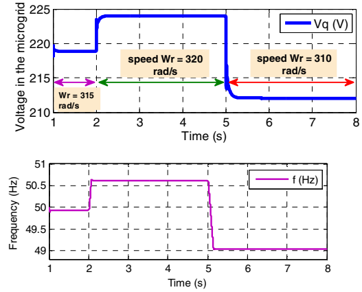
Fig. 10. Effect of wind speed variation on the voltage and frequency
