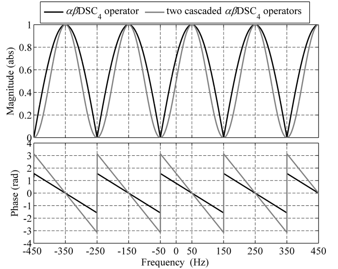
Fig. 6. Frequency response of the \alpha\beta DSC 4 operator (dark line) and two cascaded \alpha\beta DSC 4 operators (gray line).
