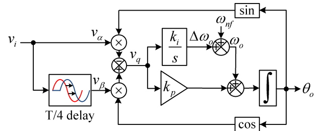
Fig. 1. Schematic of the TD-PLL.
