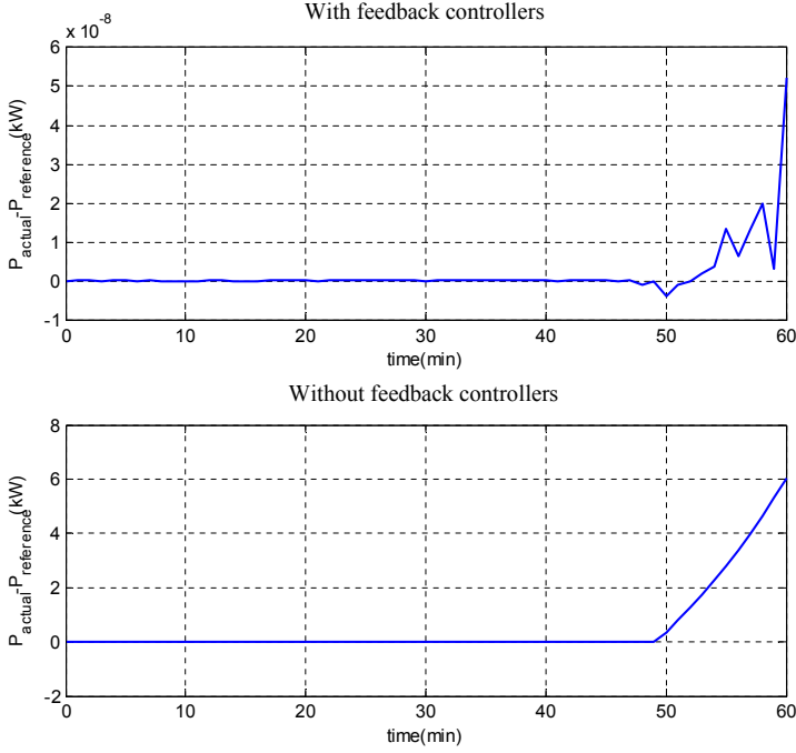
Figure 5.16: Discrepancy between the actual power consumption and the power reference for P_{reference} = 37kW , \Delta_{s_1} = \Delta_{s_2} = 10^{-5} , \Delta_{c_1} = \Delta_{c_2} = 10^{-9} . Note the different scale on the ordinate axis
