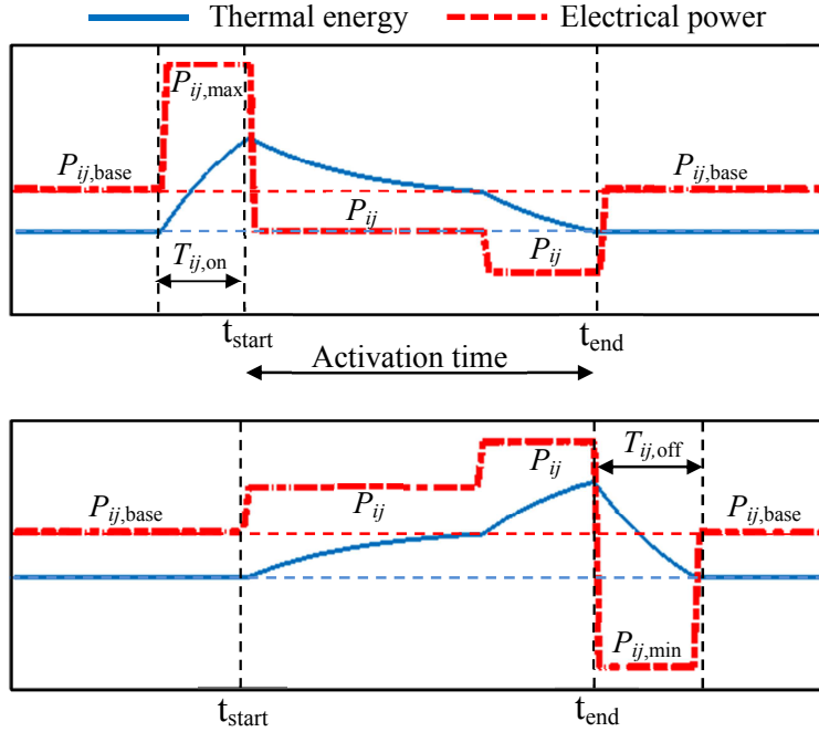
Figure 2.5: Typical power consumption profile and the stored thermal energy of the TES ij for the up-regulating (upper figure) and the down-regulating (lower figure). The interval [t_{start}, t_{end}] is called the activation time. T_{ij,on} and T_{ij,off} indicate the on-time and off-time periods respectively.
