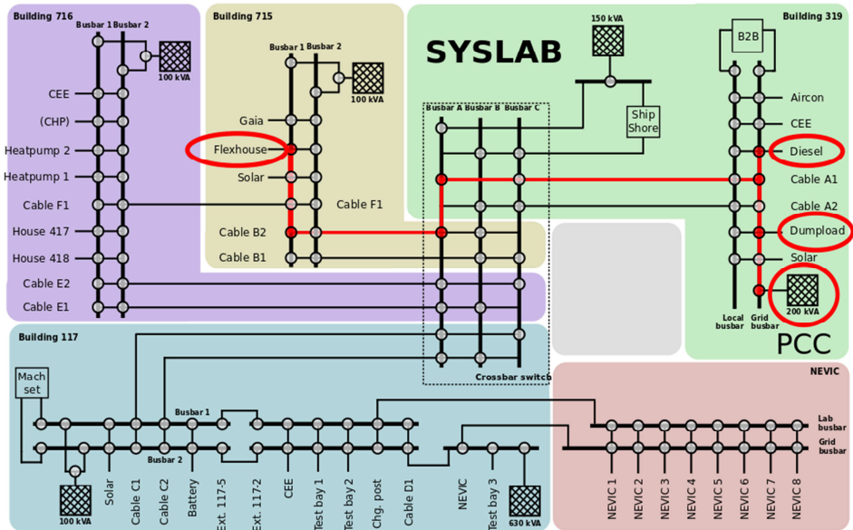
Figure 6.10: Layout of the SYSLAB test grid with active parts highlighted in red.
