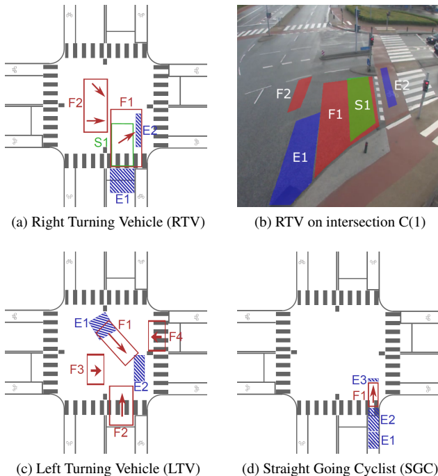
Figure 2: RTV, LTV, and SGC detectors on intersection prototypes
