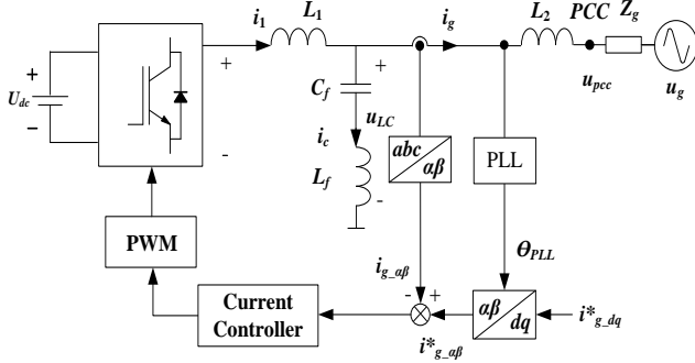
Fig. 2. LLCL -filtered converter with a single control loop.
