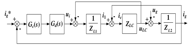
Fig. 3. Grid current control of an LLCL -filtered converter.
