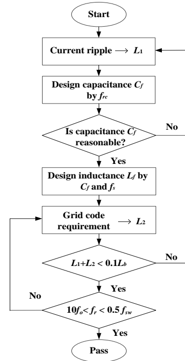
Fig. 10. Flow chart showing the parameter design procedure.
