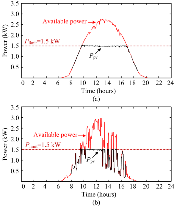
Fig. 9. Experimental results of the proposed high-performance P&O-CPG algorithm under two daily conditions: (a) clear day and (b) cloudy day.
