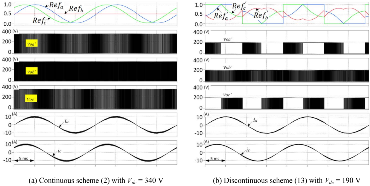
Fig. 10. Modulating references, switched voltages and terminal currents of B6 converter simulated with different modulation schemes.
