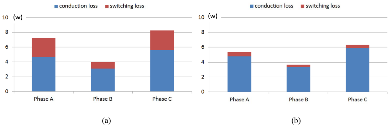
Fig. 13. Experimental loss distributions of B6 ac-dc-ac converter when modulated by (a) continuous scheme in (2) and (b) discontinuous scheme in (13).
