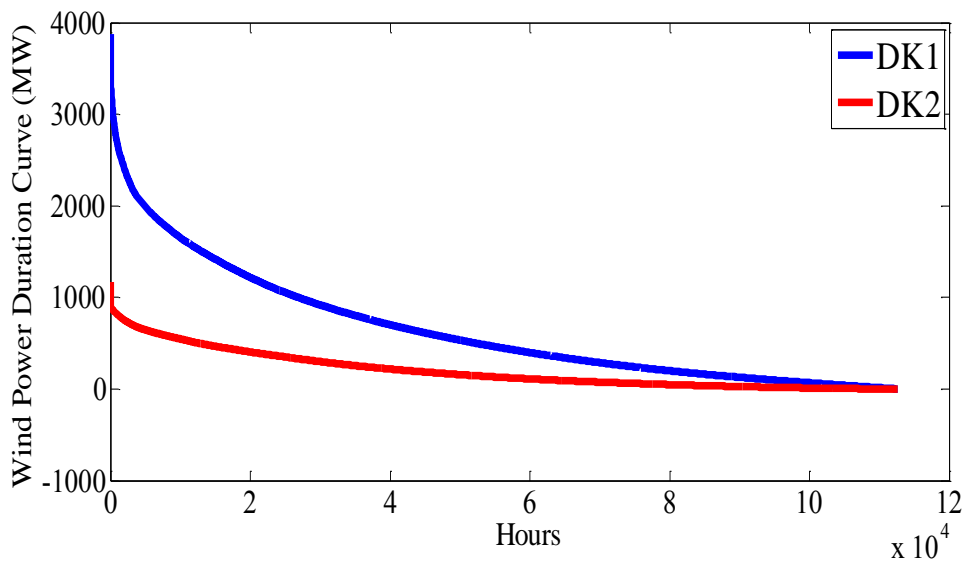
Fig. 2.6. Wind power duration curves
