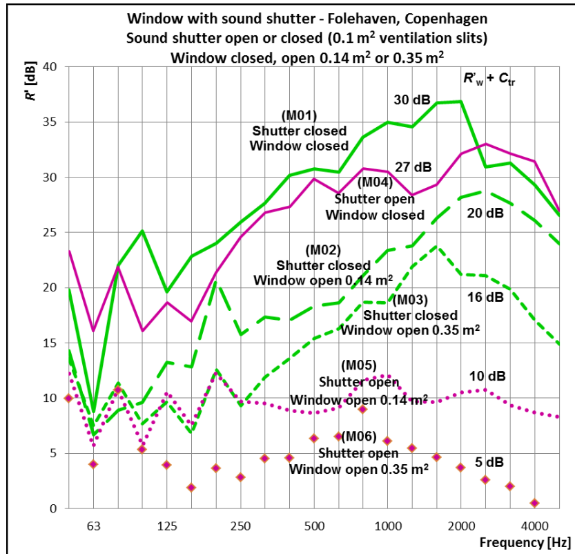
Fig. 5 – Sound insulation as a function of frequency for a window with sound shutter, both in different positions. Measurements carried out according to ISO 140-5 [12] with traffic as noise source and outdoor microphone mounted at the window, see [5].
