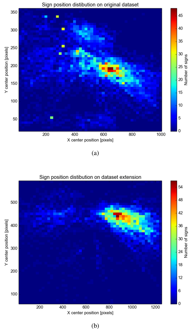
Figure 6. Heatmaps showing the positions of annotations in the frame for (a) the original dataset and (b) the extension. The contours of the road can almost be seen in the plots, especially in the extension, which has been captured using an identical camera setup for all frames. The heat maps give a very strong hint towards reasonable Regions of Interest for traffic sign detectors.
