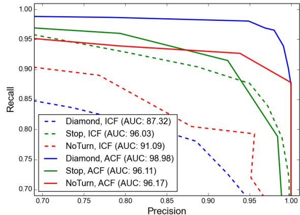
Precision-recall curve for detection of three US sign superclasses
