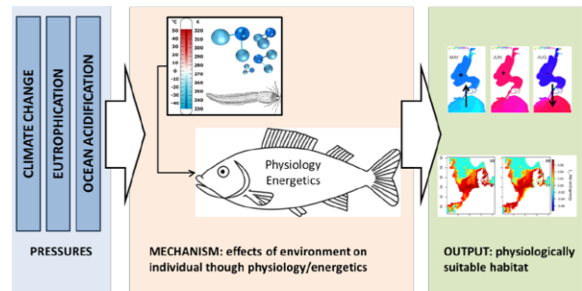
Flow chart illustrating which of the VECTORS defined drivers are relevant for this mechanism of change in species distribution, the mechanisms by which the organism is affected and the type of output that can be obtained relevant to spatial distributions.
