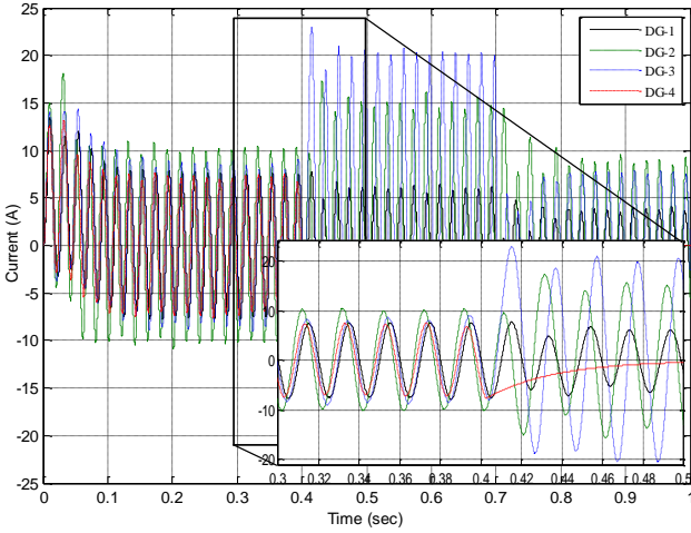
Fig. 15. The Output Current in Case 1
