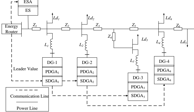
Fig. 10. Configuration of the Energy Internet Test System
