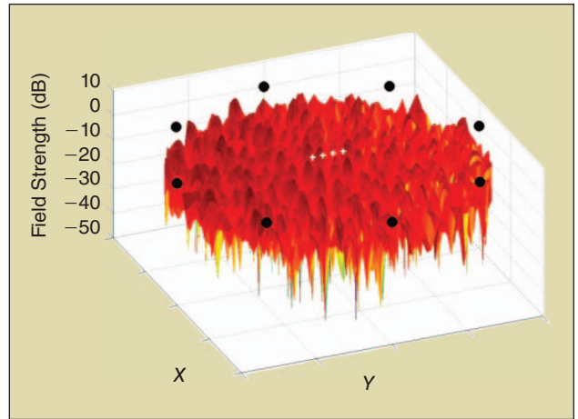
FIGURE 3 An illustration of the spatial fading channel generated with the MPAC setup, where the black dots represent the multiple probes.
