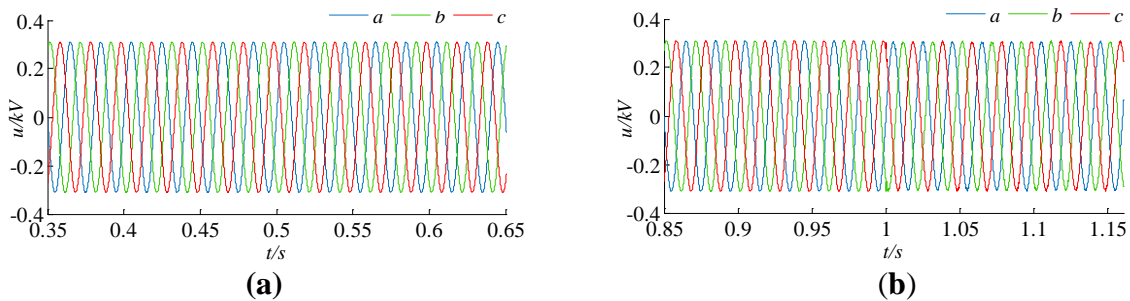
Figure 7. (a) Voltage waveform of the MSC between 0.35s~0.65s. (b) Voltage waveforms of the MSC between 0.85s~1.15s. (c) Voltage waveforms of the MSC between 1.35s~1.65s. (d) Voltage waveforms of the MSC between 1.6s~1.9s.
