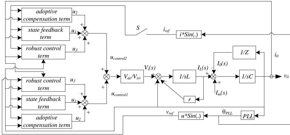
Figure 5. Block diagram of the MSC model and its ARTSMC
