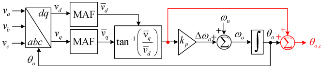
Fig. 2. Schematic diagram of the QT1-PLL.
