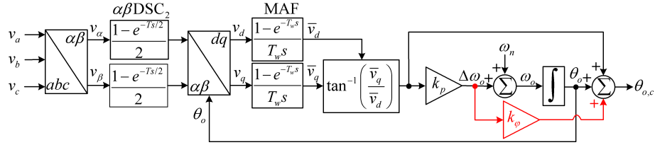
Fig. 5. Schematic diagram of HPLL.
