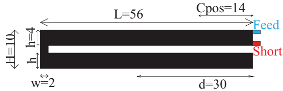
Figure 8: PIFA Geometry (dimensions in mm for M1 and M3).
