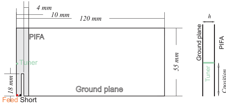
Figure 2: Antenna design (A1: h=8 mm, A2: h=2 mm) [12].
