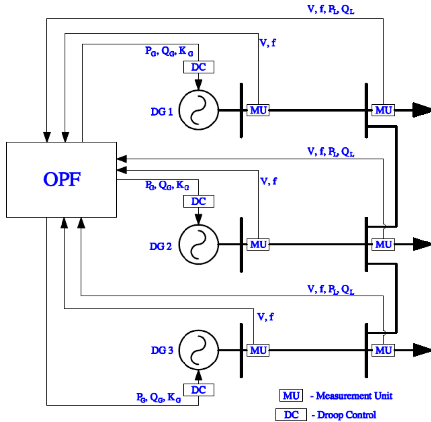
Figure 9 – General architecture of the control system
