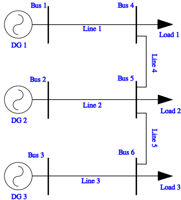
Figure 4 - The 6 bus test system
