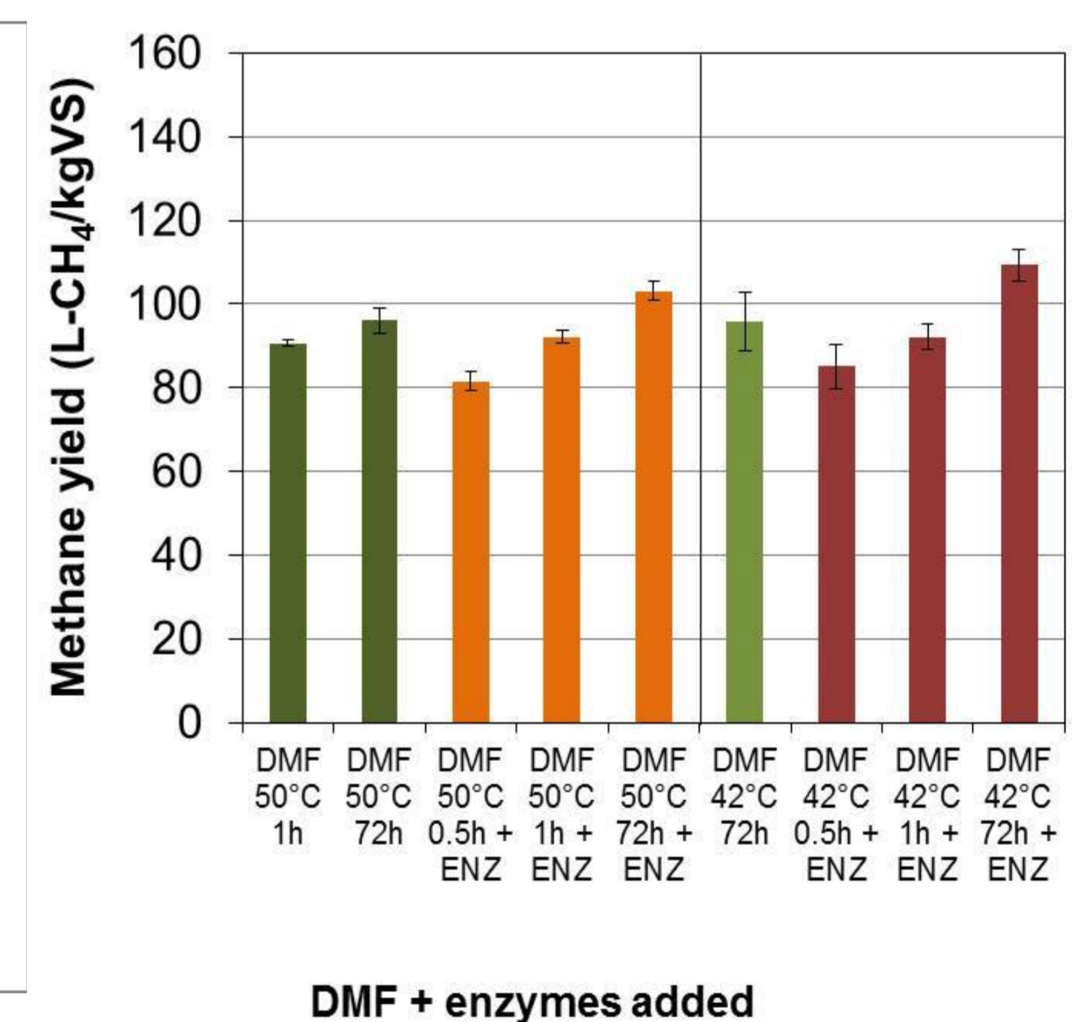
Figure 4. BMP of separated digested manure fibres, untreated and treated with enzymes (dosage 0.1% (g/g-TS), for 0.5 h at 50°C and 42°C
