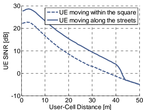
Figure 2. Signal to Interference plus Noise Ratio for users connected to a small cell in the street and a small cell in the square.
