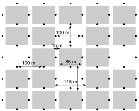
Figure 1. Small cells deployment.
