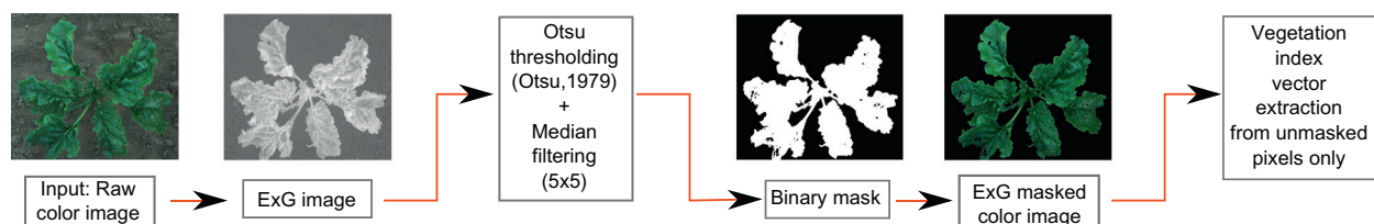
Fig. 5. Pre-Processing stages before vegetation index extraction.
