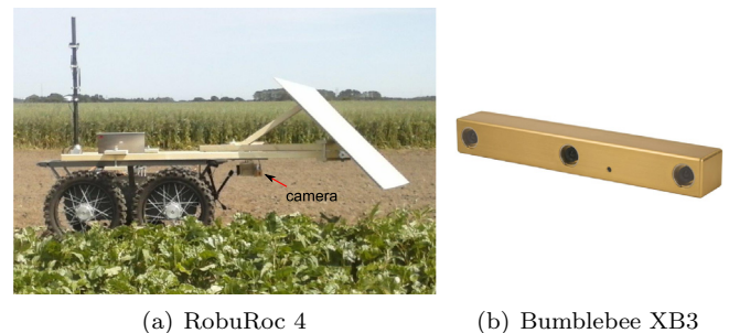
Fig. 2. Equipment: The unmanned ground vehicle (UGV) and the color camera used in the experiments. (For interpretation of the references to color in this figure legend, the reader is referred to the web version of this article.)
