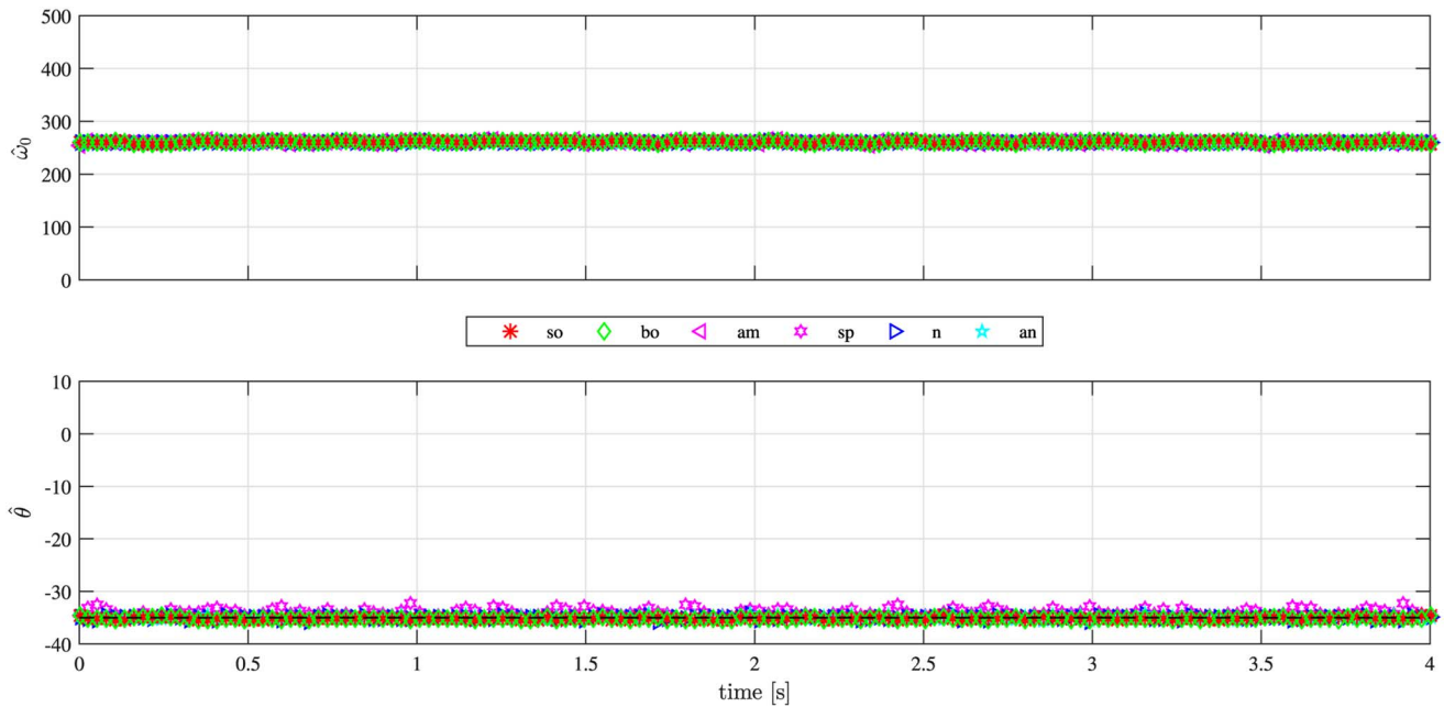
Fig. 9. Plots of (top) pitch and (bottom) DOA estimates obtained from the spatially resynthesized, trumpet signal in a scenario with no reverberation.
