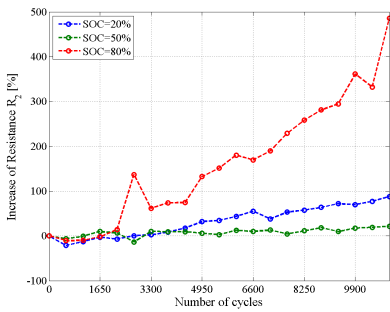
Figure E.144: Increase of resistance R_2 during accelerated calendar ageing TC3.
