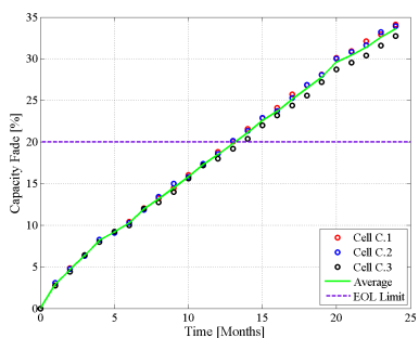
Figure E.2: Capacity fade of LFP/C battery cells subjected to Calendar 1 ageing conditions.
