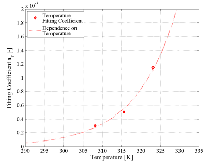
Figure E.159: Power-law relationship between the curve fitting coefficients (see Table 7.3) and the cycling temperature.
