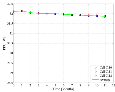
Figure E.43: Discharge PPC values measured on LFP/C cells subjected to Calendar 4 ageing conditions (RPT: SOC=80%, I_{dc}=10.A ).
