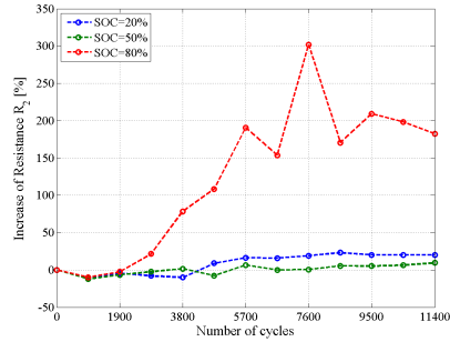
Figure E.143: Increase of resistance R_2 during accelerated calendar ageing TC2.
