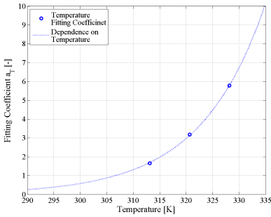
Figure E.81: Exponential relationship between the curve fitting coefficients (see Table 6.5) and the storage temperature.
