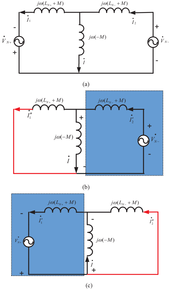
Fig. 5. Equivalent circuits of the zero sequence blocking transformers: (a) decoupled equivalent circuit, (b) equivalent circuit ( N_+ short circuit), and (c) equivalent circuit ( N_- short circuit).
