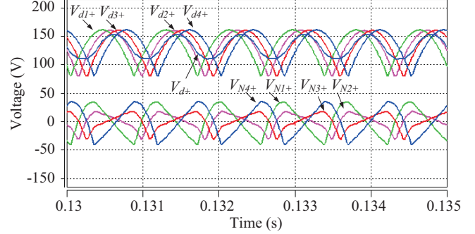
Fig. 4. Voltages across the zero sequence blocking transformers.
