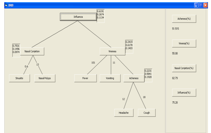
Fig. 3. BRBES's Interface
