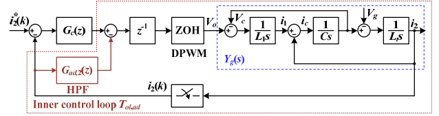
Fig. 6. Block diagram of grid current control loop in the discrete z -domain.
