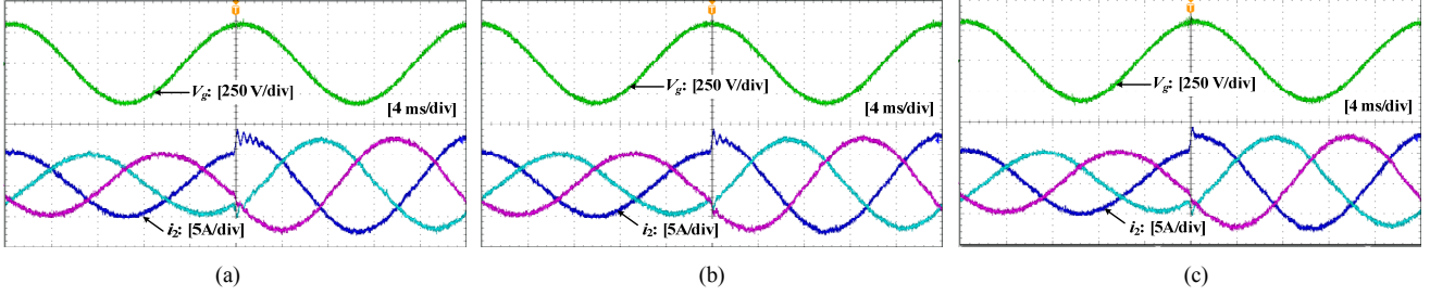
Fig. 11. Measured A-phase grid voltage and grid current for C_f = 4.7 \mu\text{F} , \omega_{res} = 0.24\omega_s . (a) k_{ad} = 0 . (b) k_{ad} = 5 , \omega_{ad} = 0.35\omega_s . (c) k_{ad} = 15 , \omega_{ad} = 0.35\omega_s .
