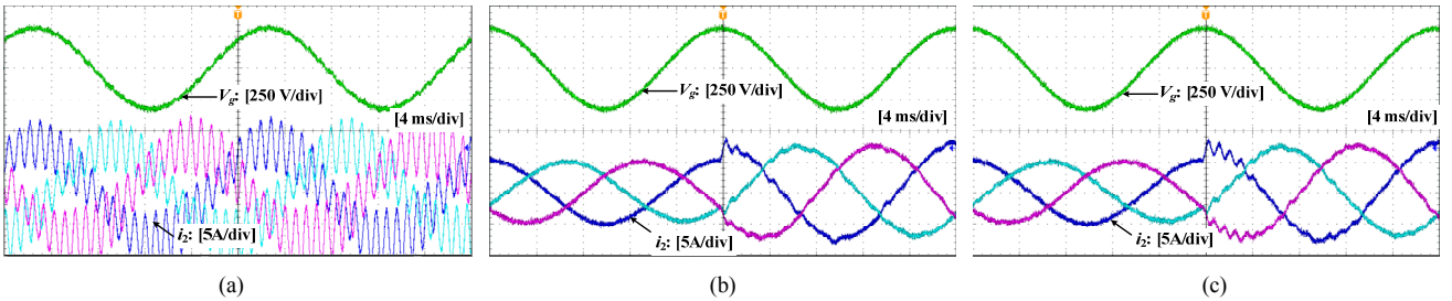
Fig. 13. Measured A-phase grid voltage and grid current for C_f = 14.1 \mu\text{F} , \omega_{res} = 0.14\omega_s . (a) k_{ad} = 5 , \omega_{ad} = 0.15\omega_s . (b) k_{ad} = 15 , \omega_{ad} = 0.15\omega_s . (c) k_{ad} = 15 , \omega_{ad} = 0.25\omega_s .
