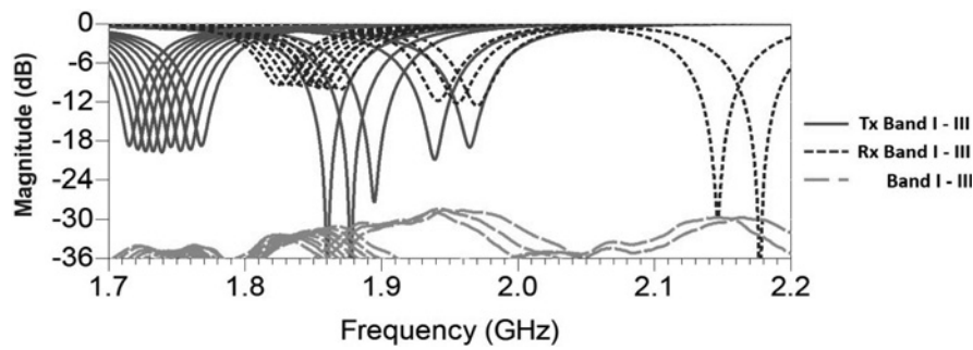
Fig. 16 Measured scattering parameters Reflection coefficients ( S_{11} , S_{22} ) and coupling coefficient ( S_{21} ) of the Tx and Rx antennas
